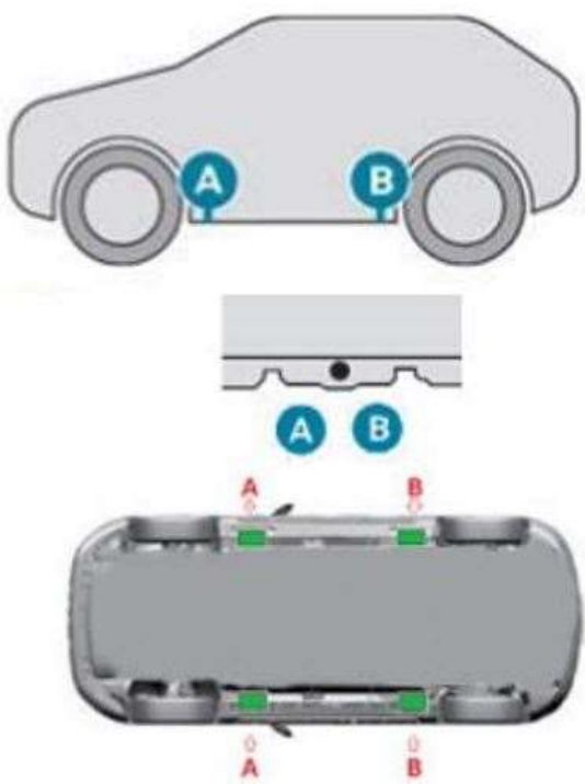
Stabilization/lifting points
